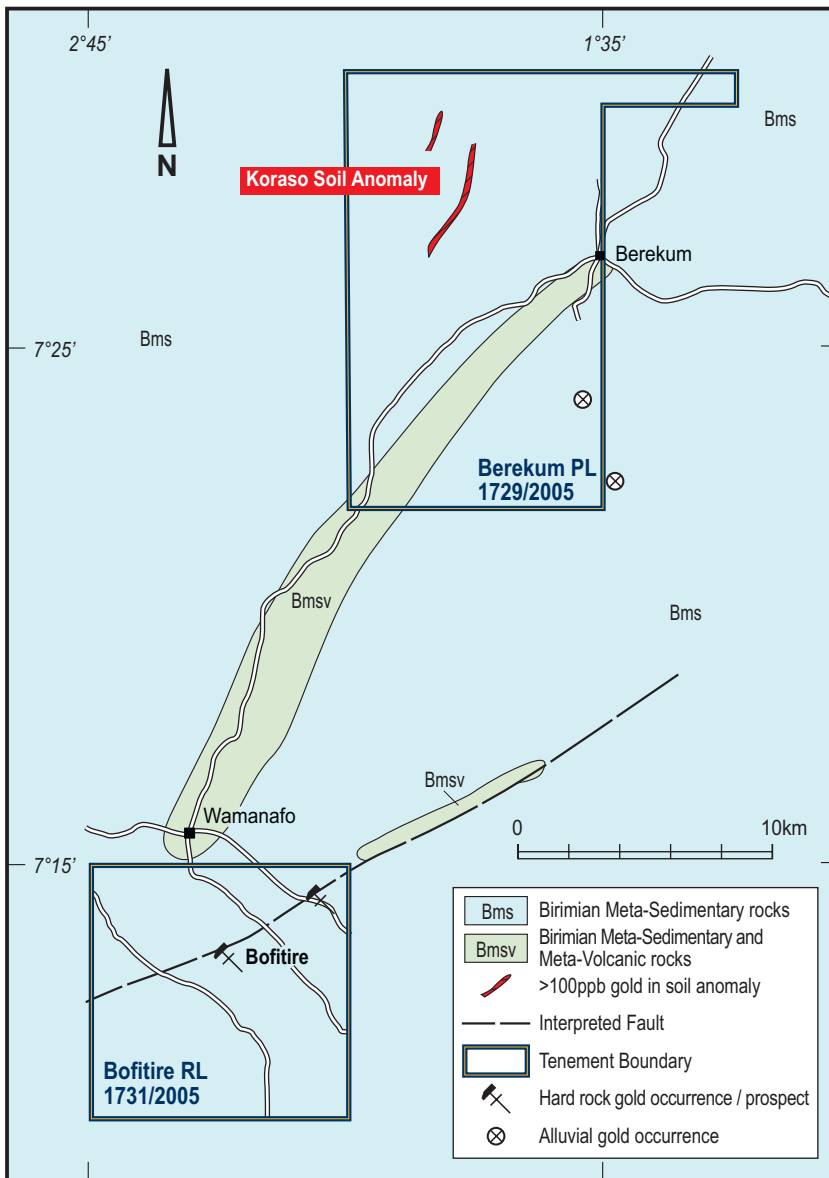
Figure 8 CASTLE MINERALS LIMITED SUNYANI BASIN PROJECT TENEMENTS AND GEOLOGY
